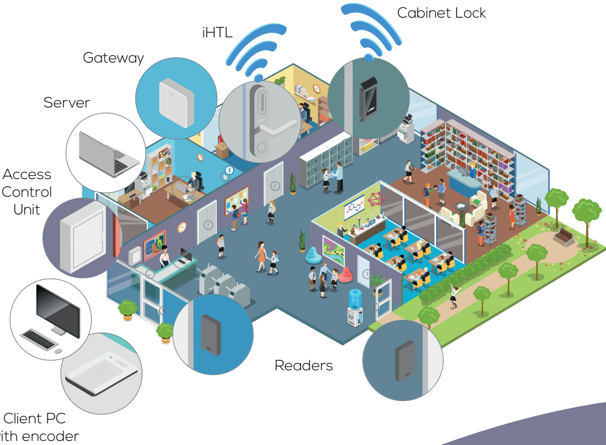
Example hybrid system with wired readers and bluetooth handle sets
